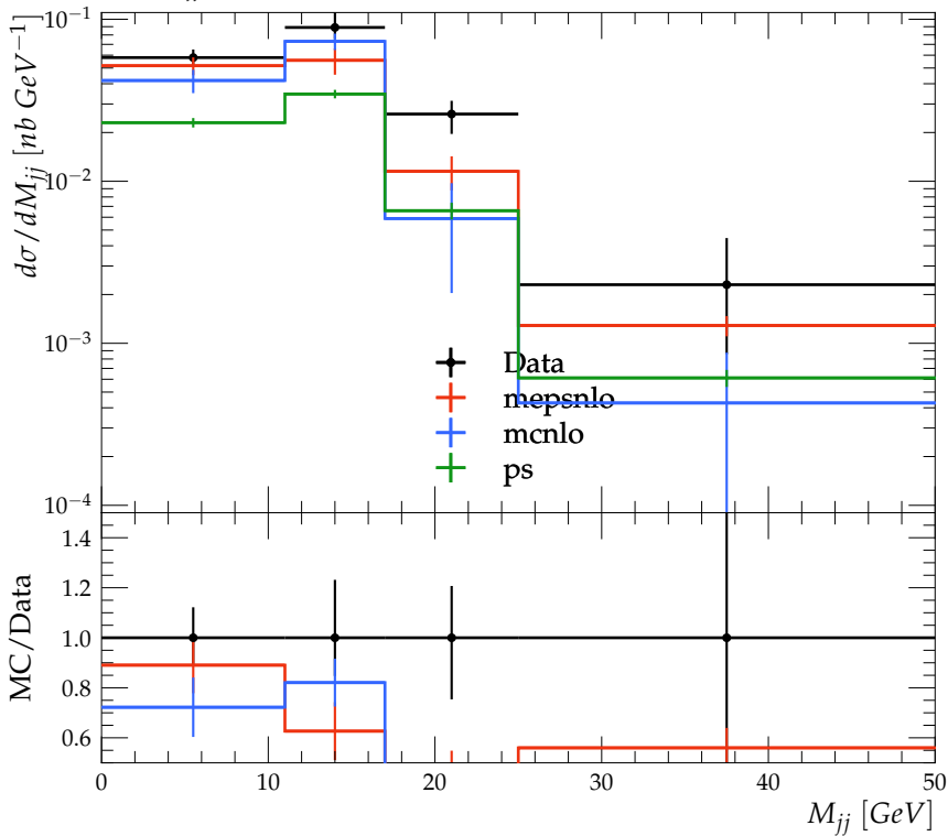
d\sigma/dM_{jj} for D^{*\pm} production with dijets (Breit frame)
