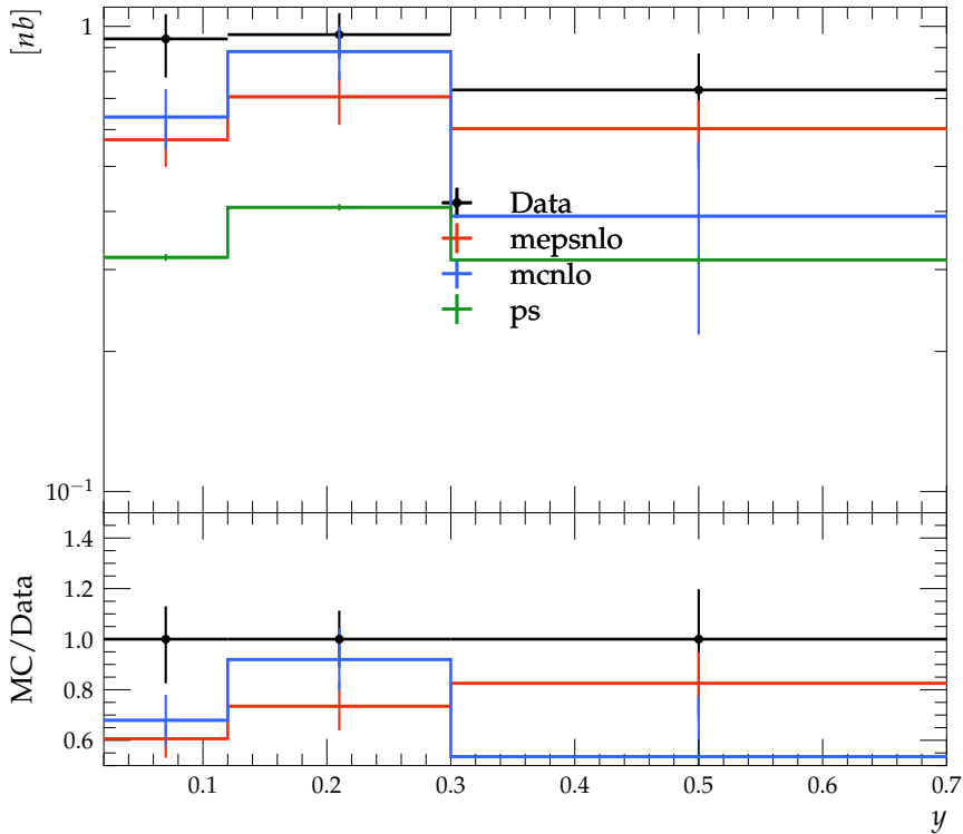
Differential cross-section of D^\pm meson production for 9.0 < Q^2 < 44.0
