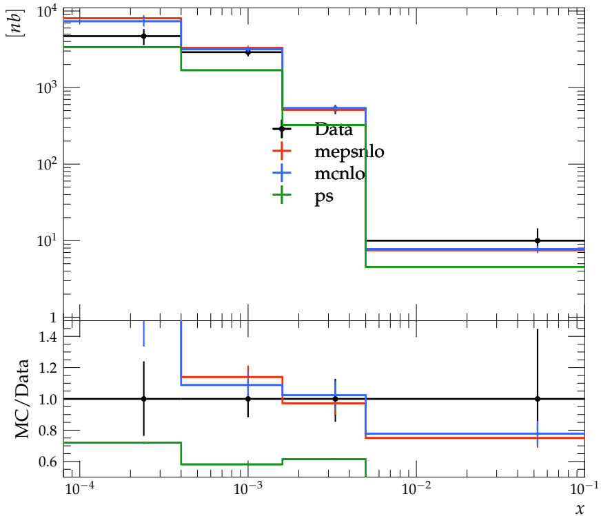
Differential cross-section of D^0 meson production
