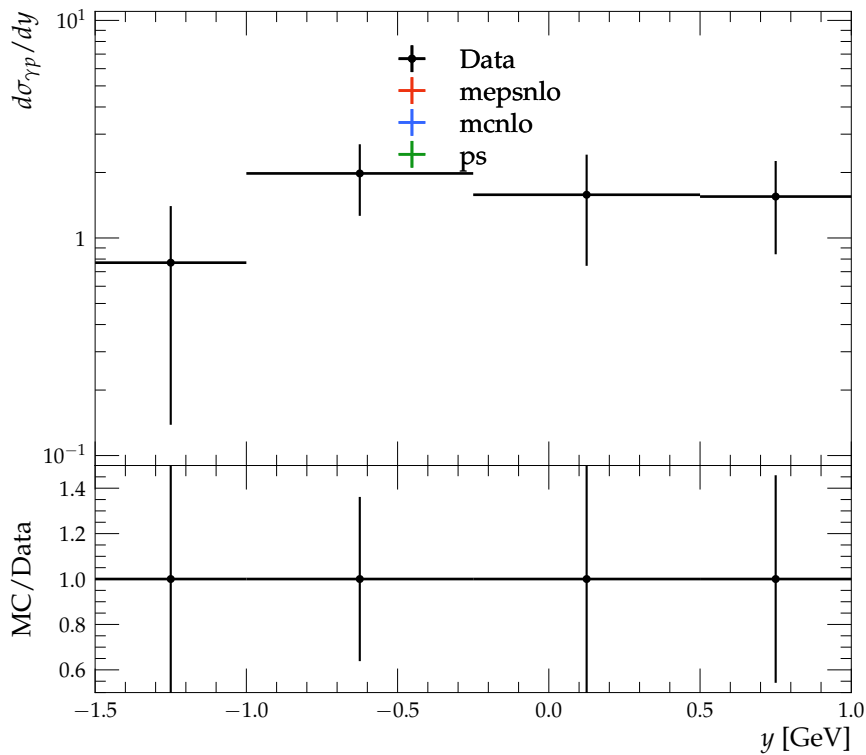
Double-differential cross section 5.0\text{GeV} < p_T < 10.5\text{GeV}
