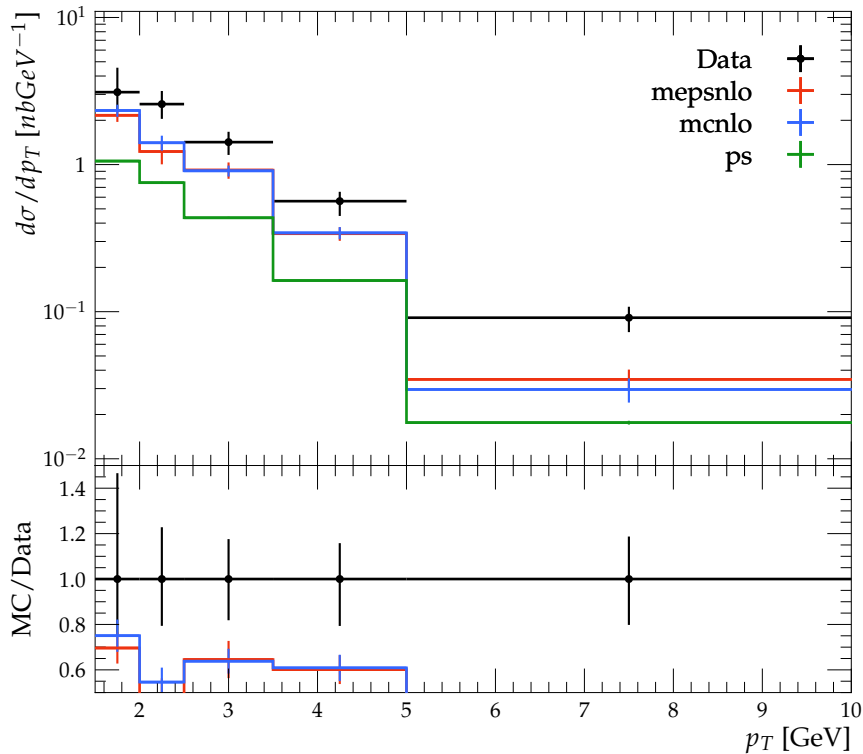
Transverse D* momentum lab frame
