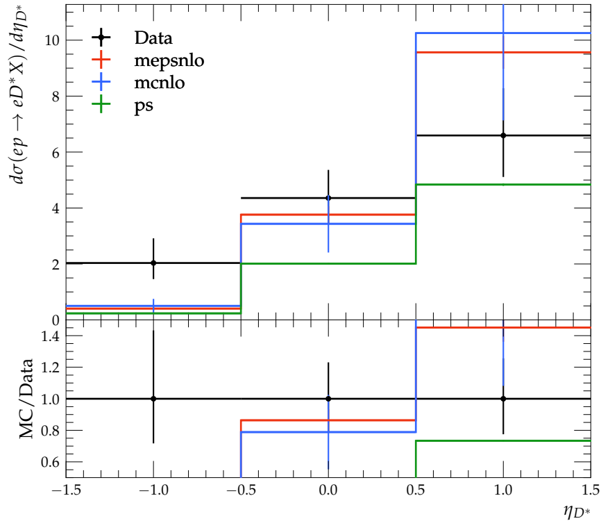
D^* production in DIS (H1) z_D < 0.25
