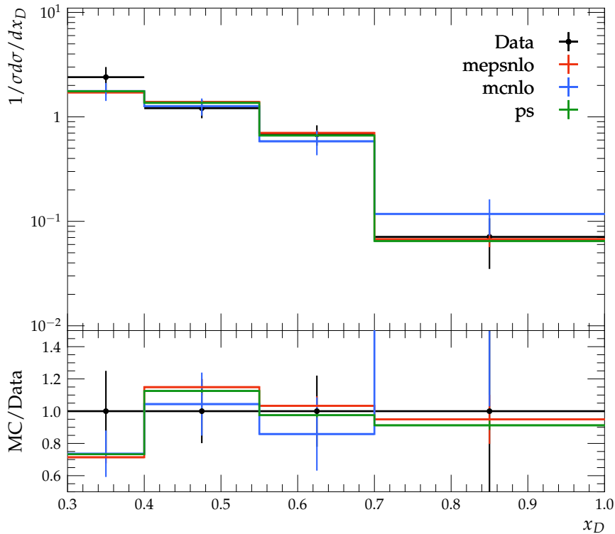
Normalized x_D Distribution for D^0
