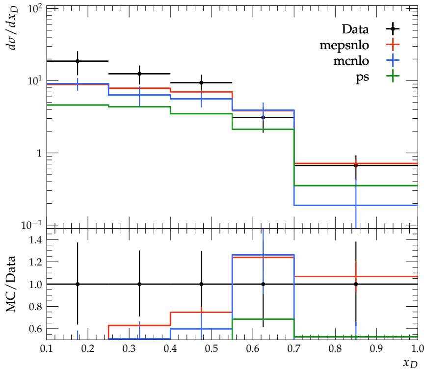
x_D Distribution for D^*
