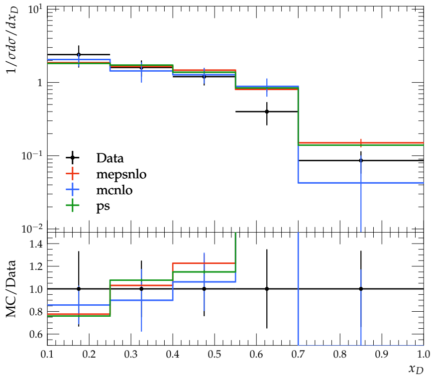
Normalized x_D Distribution for D^*
