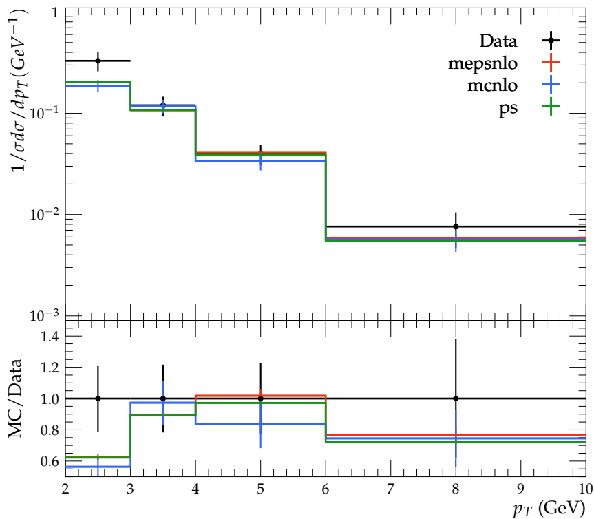
Normalized Differential Cross Section for D^0
