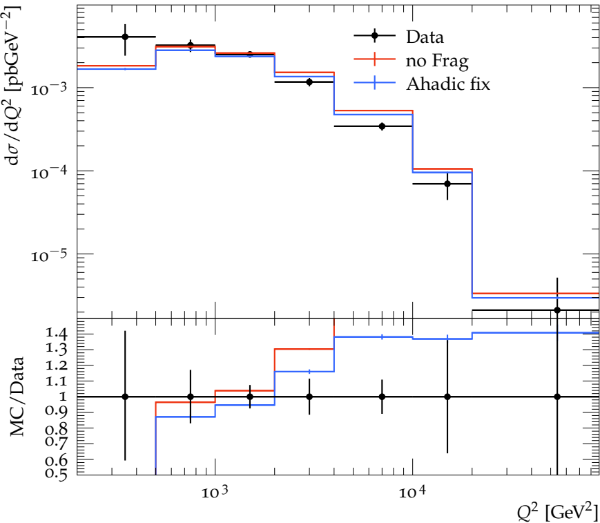
Unpolarized inclusive two jet cross section vs Q^2 , e^-
