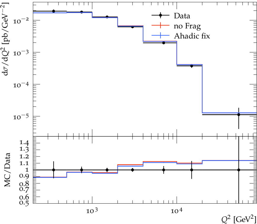
Unpolarized inclusive jet cross section vs Q^2, e^-
