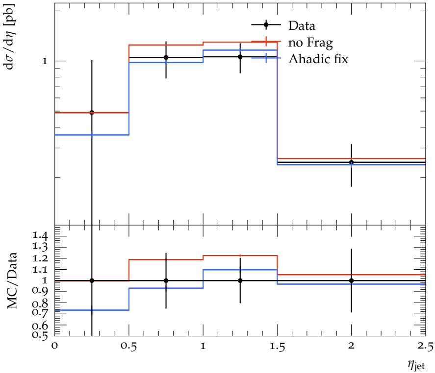
Unpolarized inclusive three jet cross section vs jet \eta , e^-
