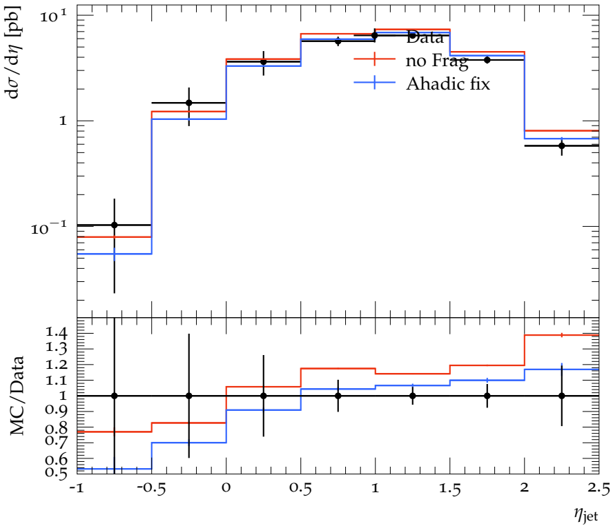
Unpolarized inclusive two jet cross section vs jet \eta , e^-
