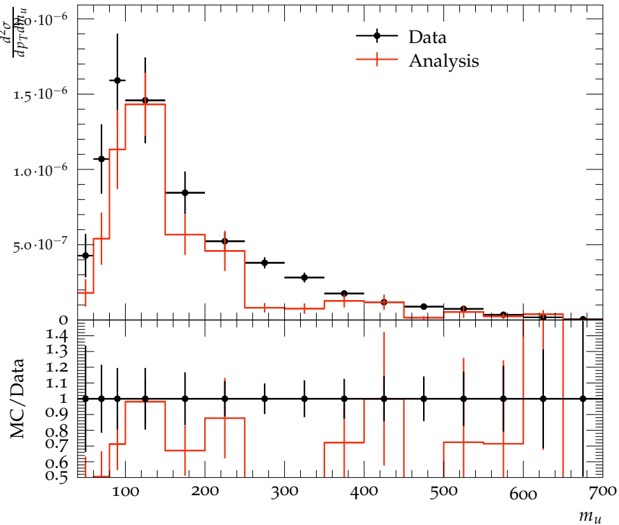
CMS, 13 TeV, Ungroomed jet mass m_u ( p_T > 1300 GeV)
