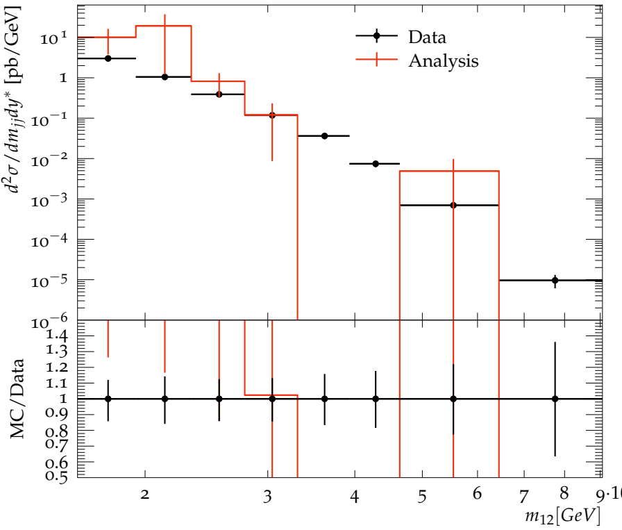
Dijet cross section ( 2.5 \leq y^* < 3.0 ), R=0.4
