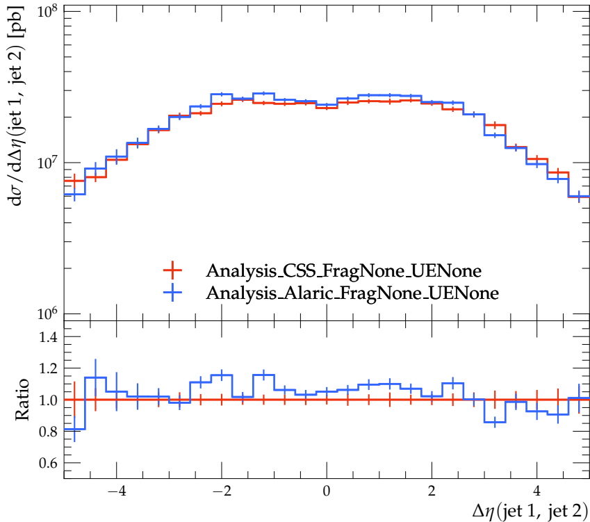
Pseudorapidity separation between jets
