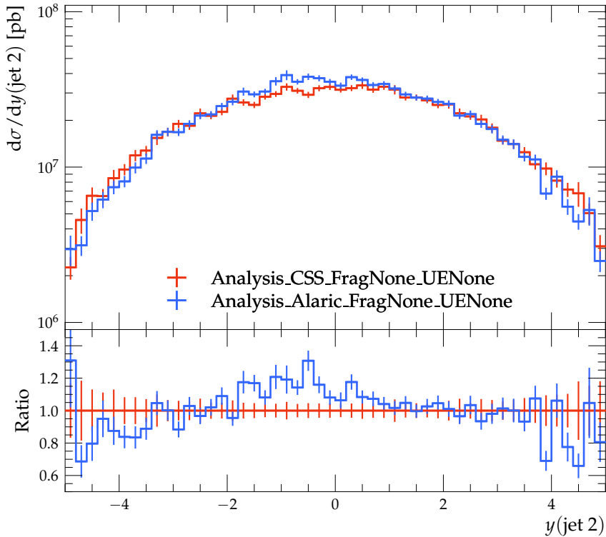
Rapidity of second jet
