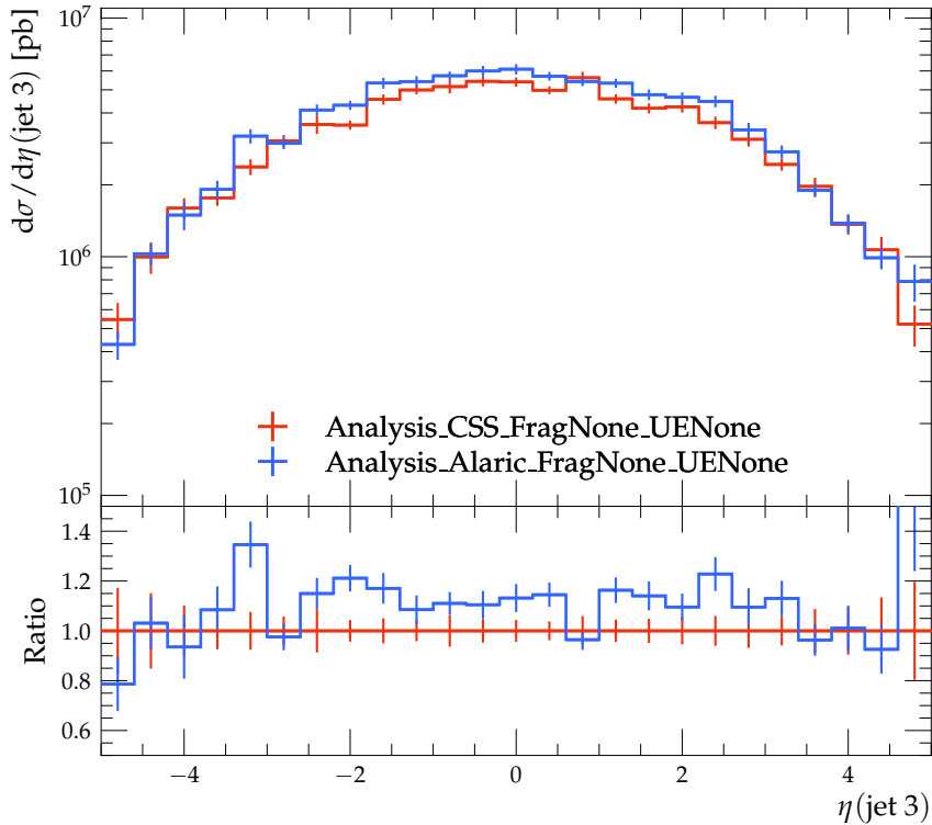
Pseudorapidity of third jet
