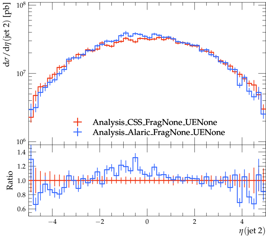
Pseudorapidity of second jet
