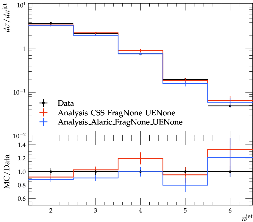
Jet multiplicity for H_{T2} > 2.0 TeV
