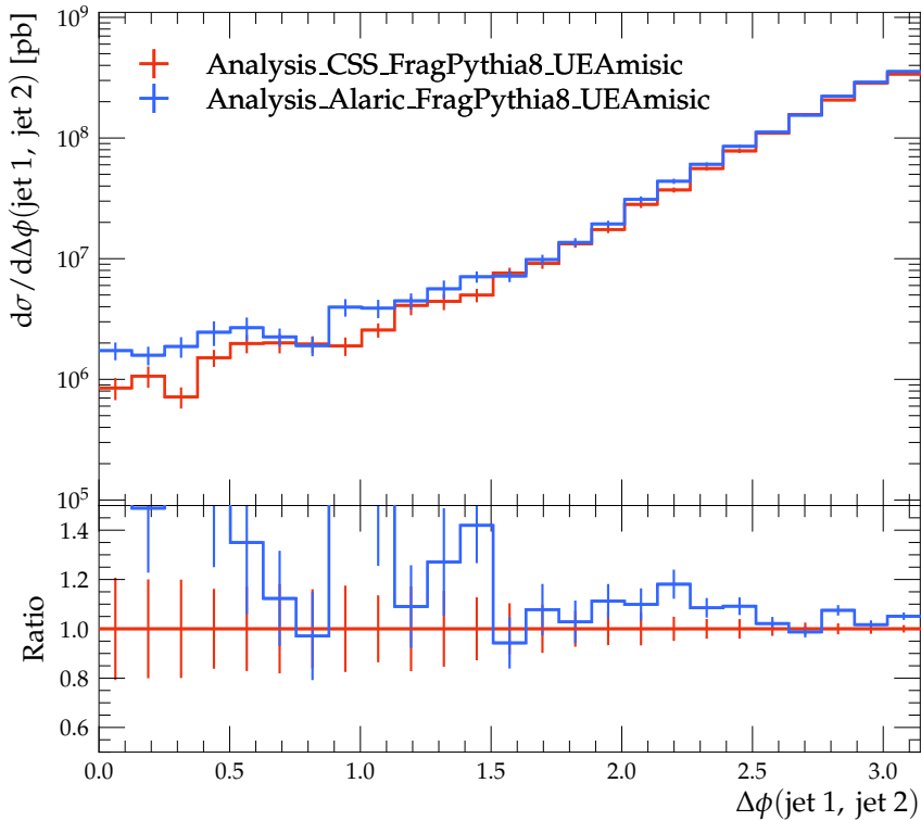
Azimuthal separation between jets
