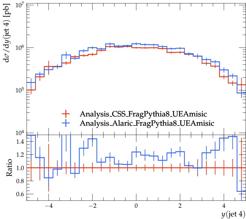
Rapidity of fourth jet
