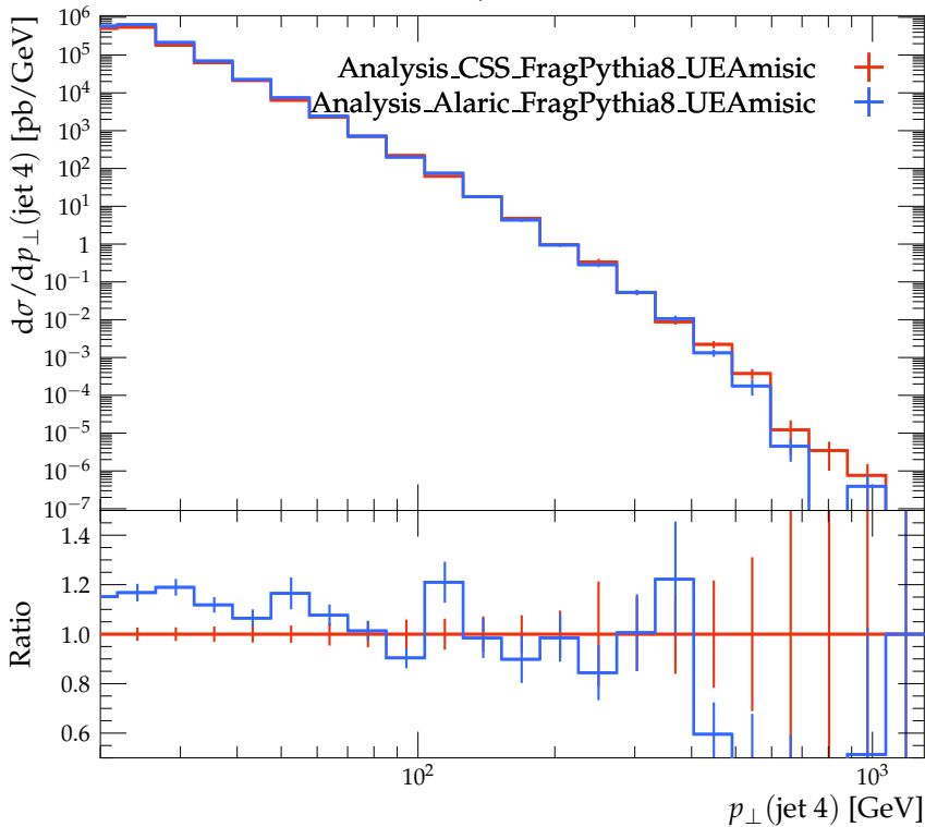
Transverse momentum of fourth jet
