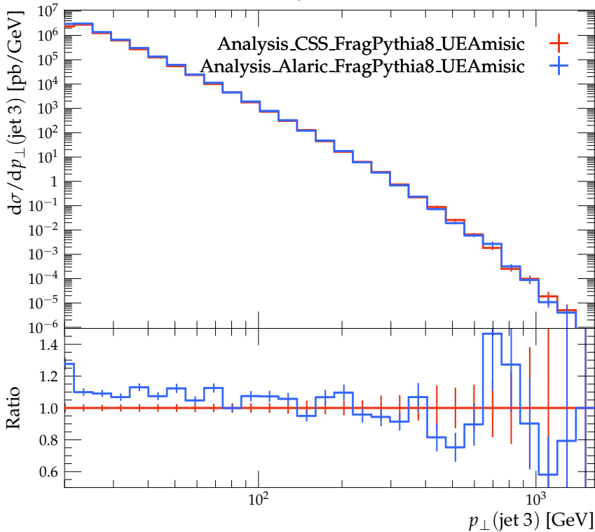
Transverse momentum of third jet
