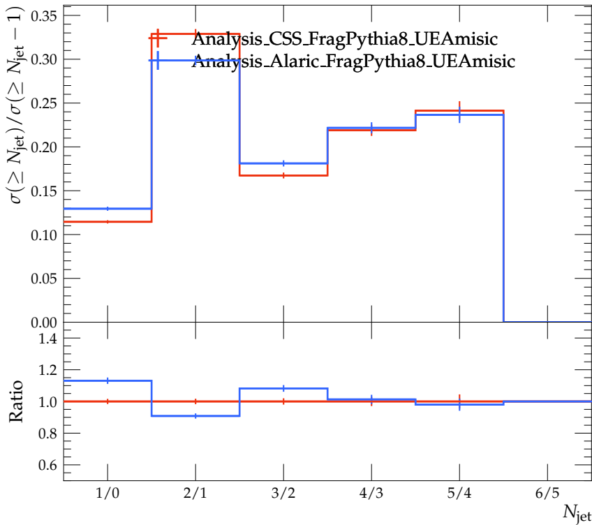
Ratio of jet multiplicity
