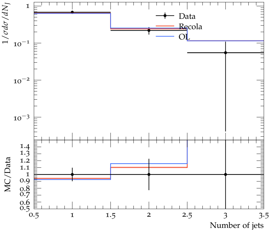
CMS, 13 TeV, W^+W^- , Figure 7
