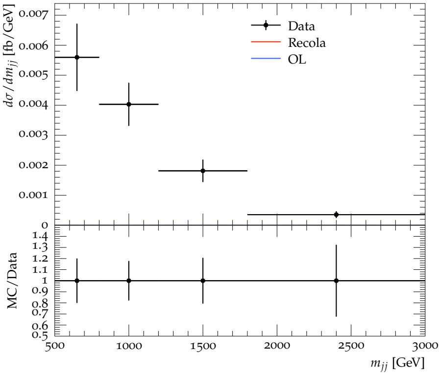
CMS, 13 TeV, WZjj, Figure 5 left
