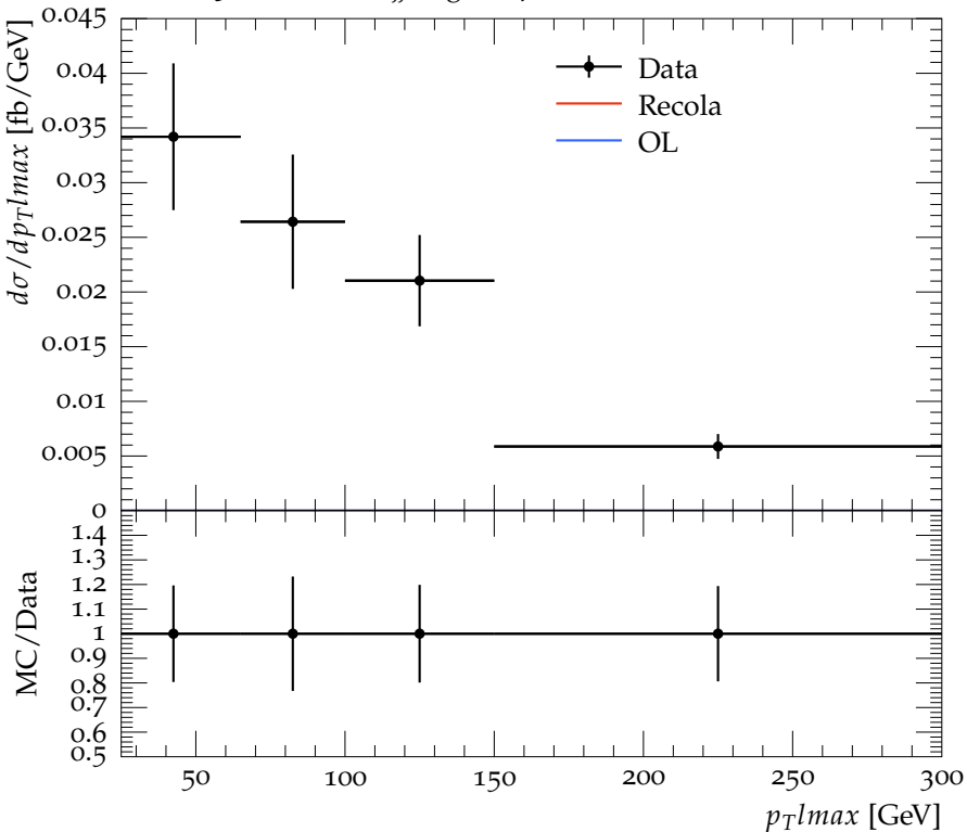
CMS, 13 TeV, W^+W^+jj , Figure 4 lower left
