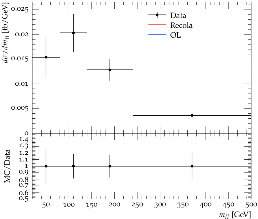
CMS, 13 TeV, W^+W^+jj , Figure 4 middle left
