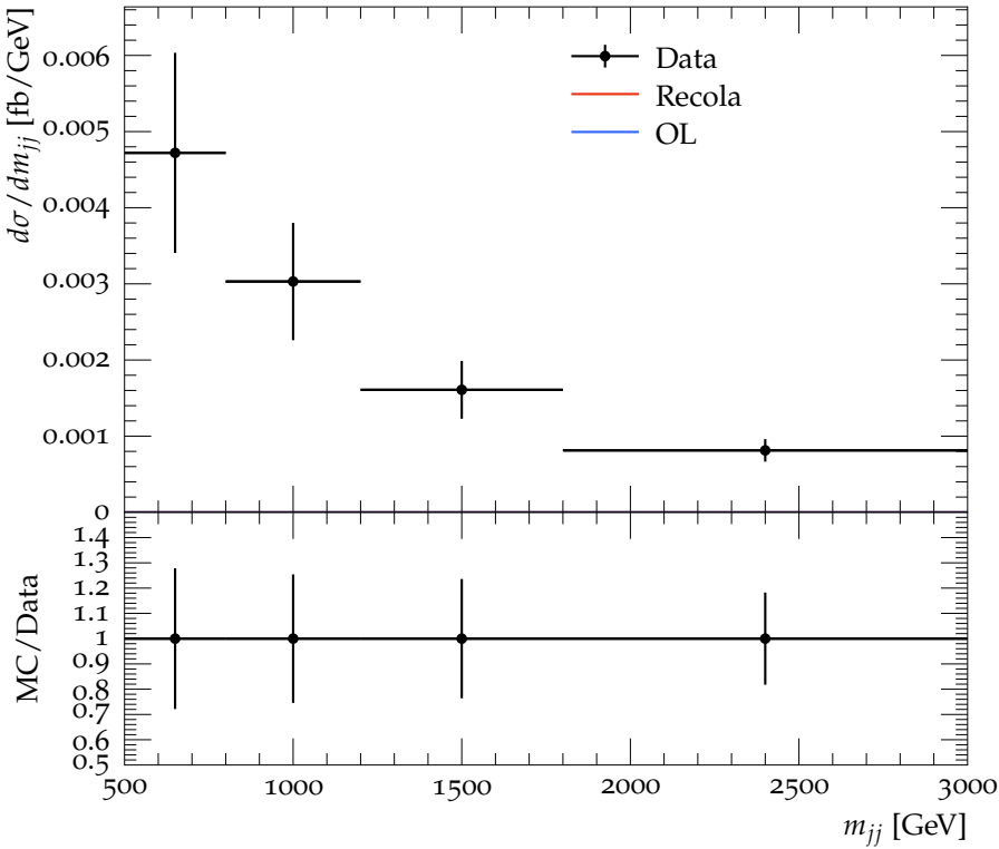
CMS, 13 TeV, W^+W^{+jj} , Figure 4 upper left
