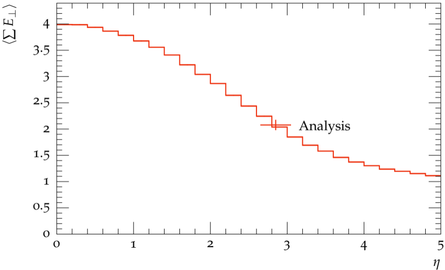
Pseudorapidity distribution of \langle \sum E_{\perp} \rangle
