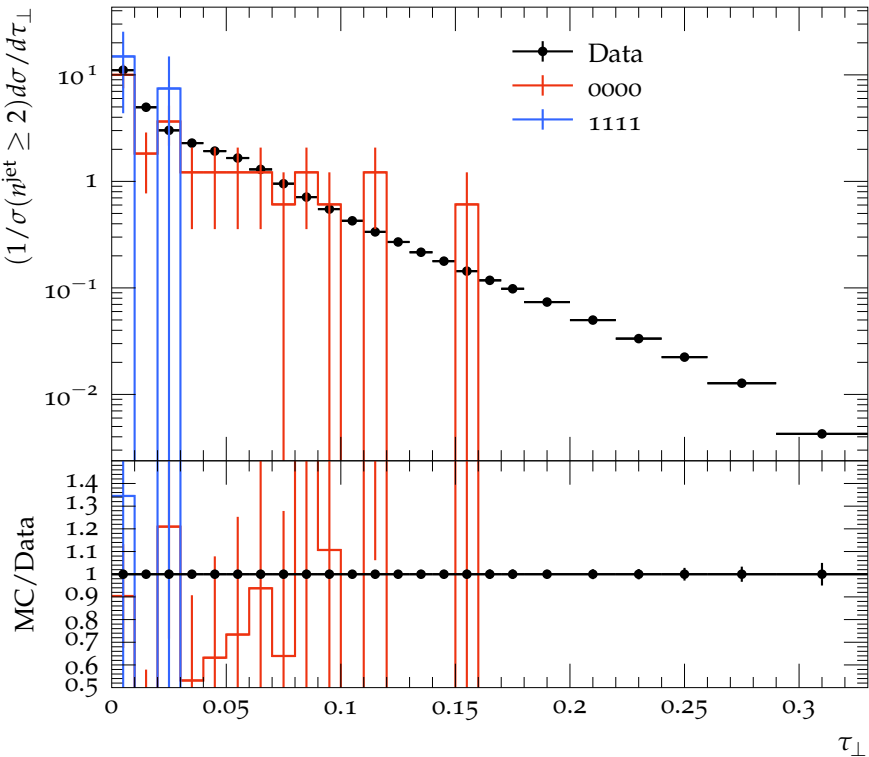
Transverse Thrust for n^{\text{jet}} = 3, 1.5 \text{ TeV} < H_{T2} < 2.0 \text{ TeV}
