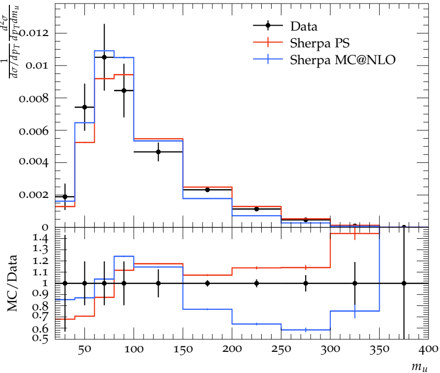
CMS, 13 TeV, Ungroomed jet mass m_u ( 650 < p_T < 760 GeV)
