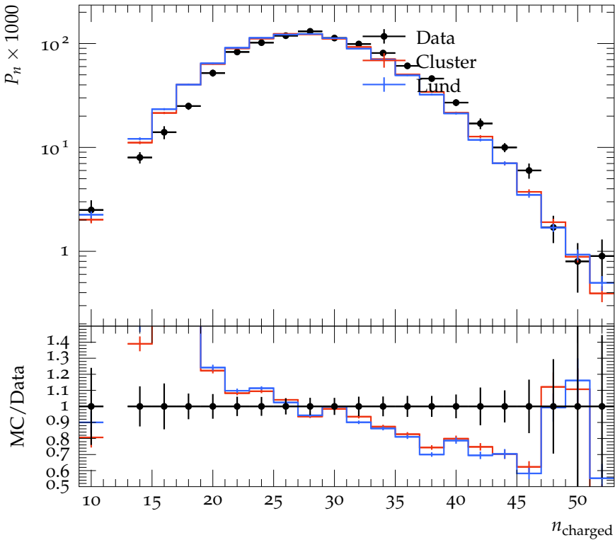
Charged particle multiplicity, 4-jets, y_{\text{cut}} = 0.02
