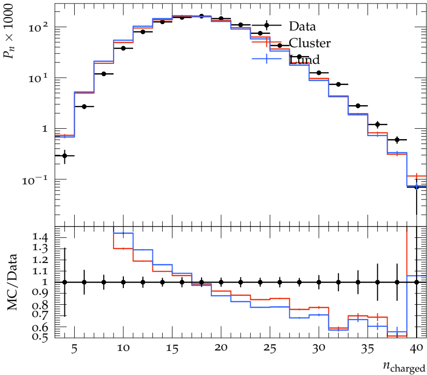
Charged particle multiplicity, 2-jets, y_{\text{cut}} = 0.02
