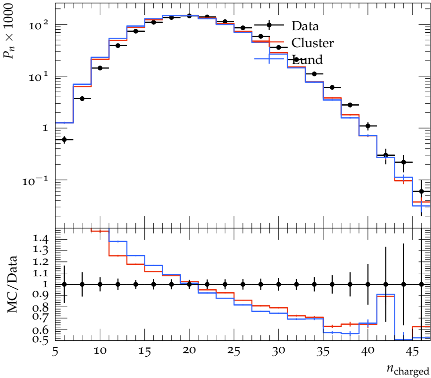
Charged particle multiplicity, 3-jets, y_{\text{cut}} = 0.01
