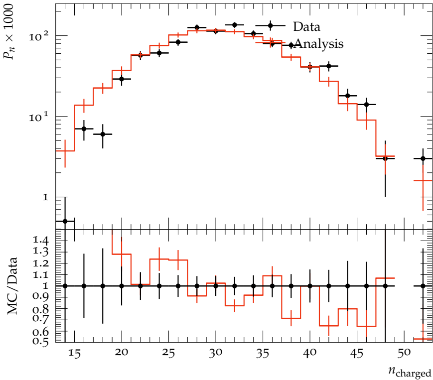
Charged particle multiplicity, 4-jets, y_{\text{cut}} = 0.04
