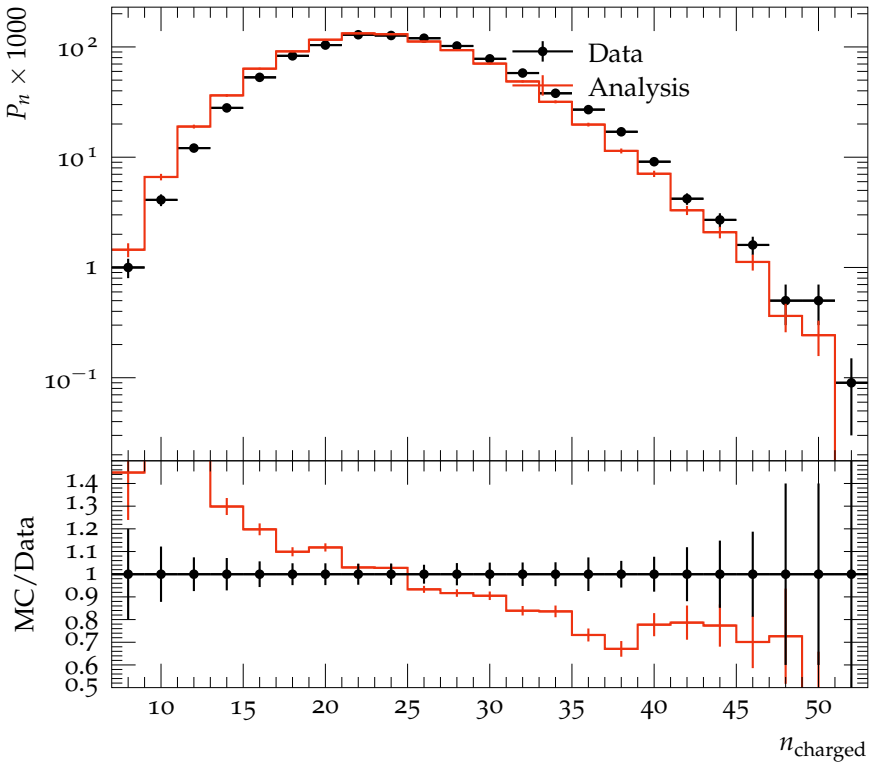
Charged particle multiplicity, 3-jets, y_{\text{cut}} = 0.04
