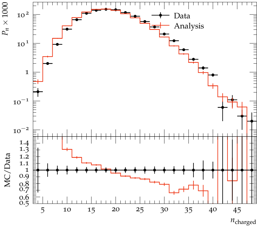
Charged particle multiplicity, 2-jets, y_{\text{cut}} = 0.04
