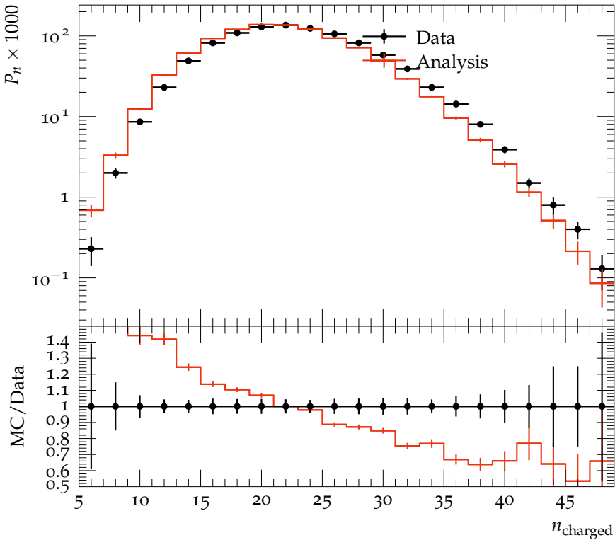
Charged particle multiplicity, 3-jets, y_{\text{cut}} = 0.02
