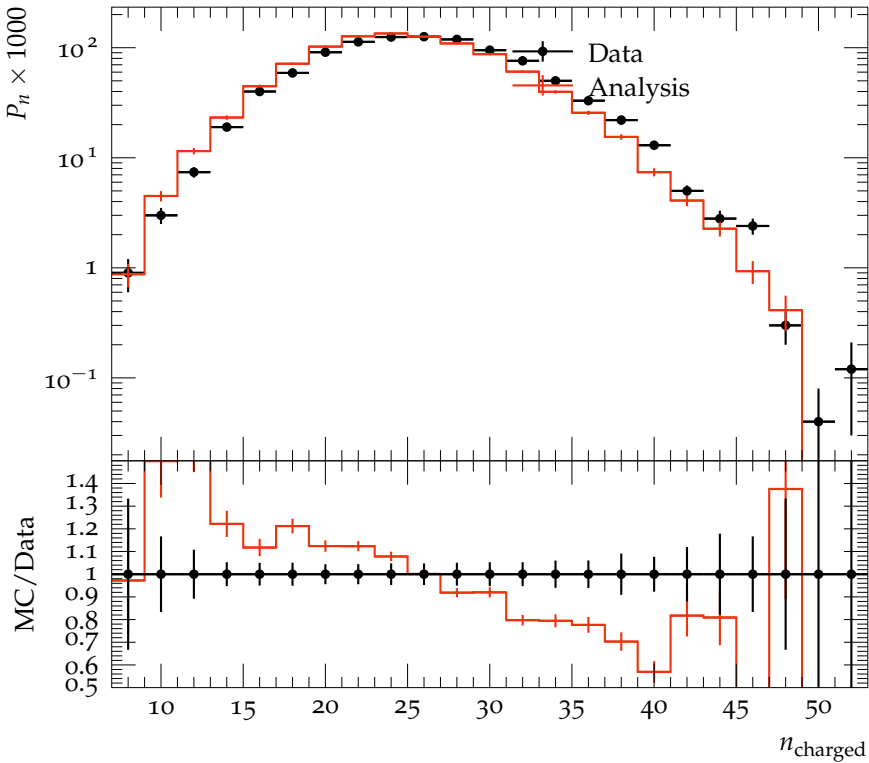
Charged particle multiplicity, 4-jets, y_{\text{cut}} = 0.01
