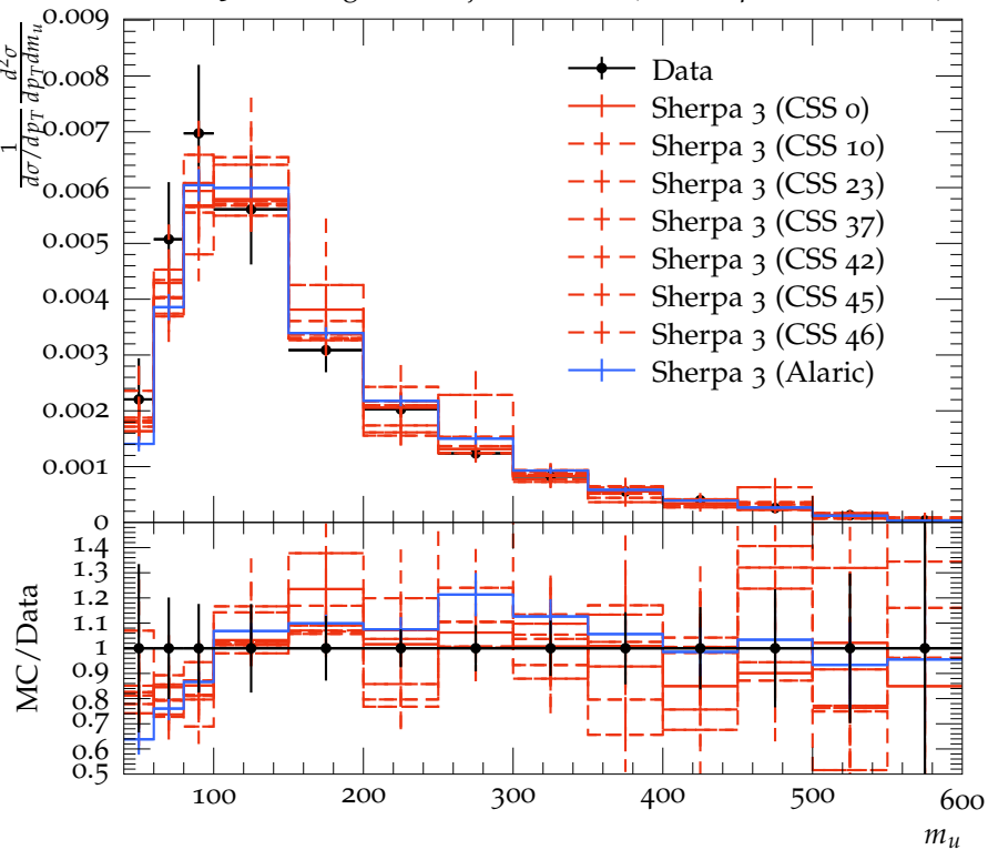
CMS, 13 TeV, Ungroomed jet mass m_u ( 1200 < p_T < 1300 GeV)
