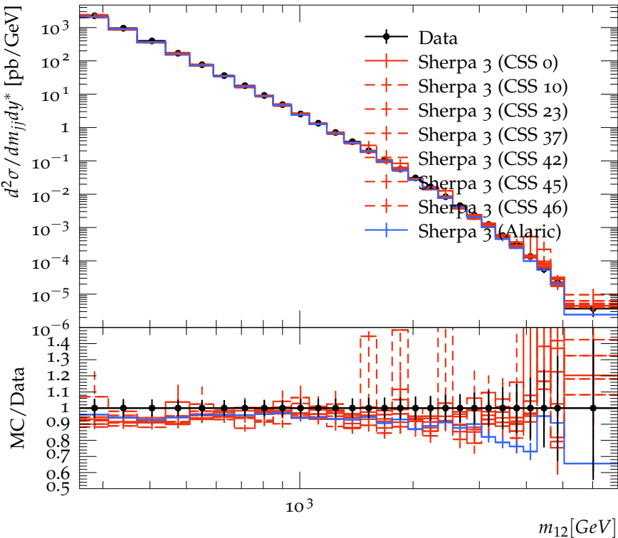
Dijet cross section ( y^* < 0.5 ), R=0.4
