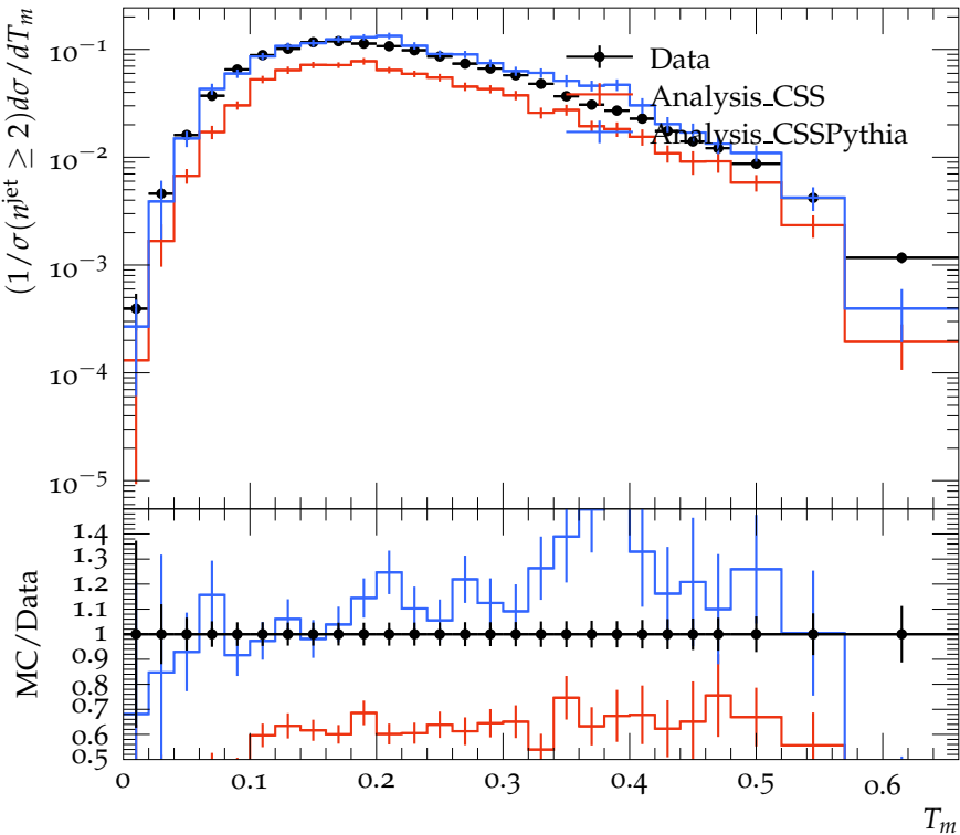
Thrust Minor for n^{\text{jet}} = 5 , H_{T2} > 2.0 TeV
