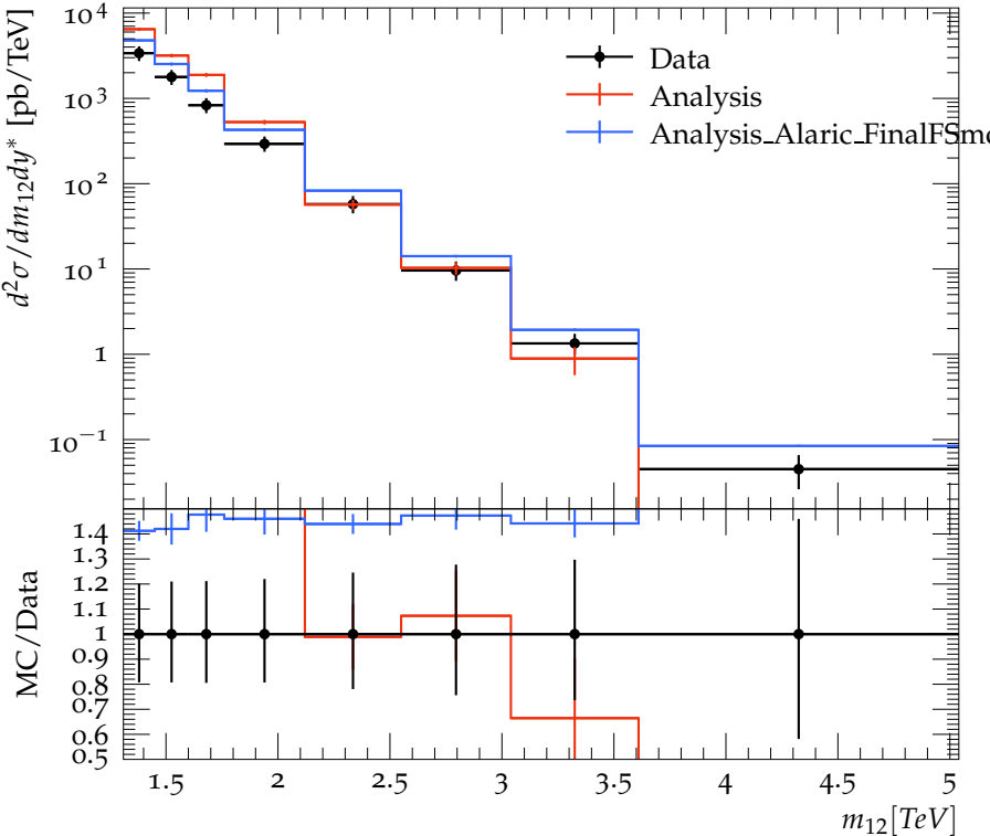
Dijet double-differential cross sections ( 2.0 < y^* < 2.5 ), R=0.6
