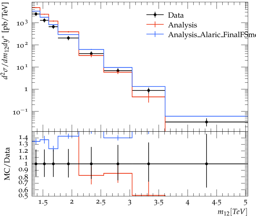
Dijet double-differential cross sections ( 2.0 < y^* < 2.5 ), R=0.4
