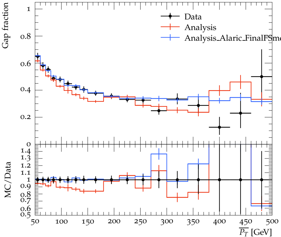
Gap fraction vs \overline{P_T} for 3.0 < |\Delta y| < 4.0 , Leading Jet
