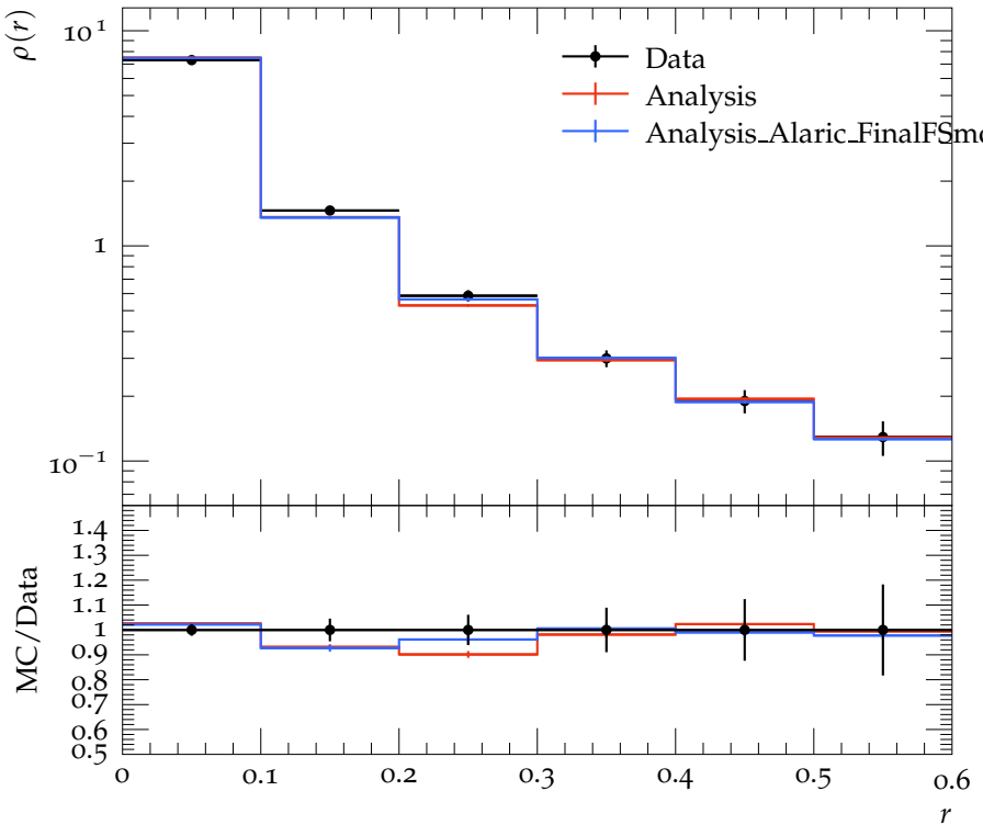
Jet shape \rho for p_{\perp} \in 160\text{--}210 GeV, y \in 2.1\text{--}2.8
