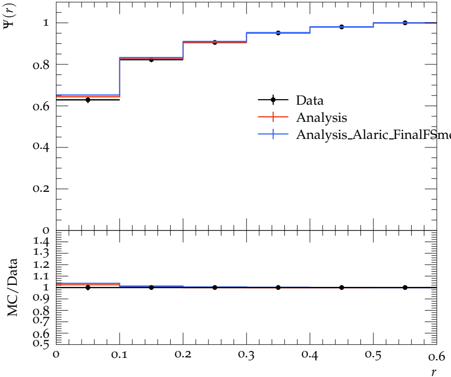
Jet shape \Psi for p_{\perp} \in 110\text{--}160\text{ GeV} , y \in 0.0\text{--}2.8
